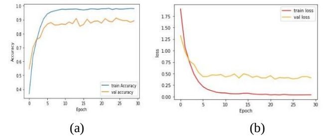
Figure 4. (a) Accuracy curve (b) Loss curve of 39 LFCC Features
